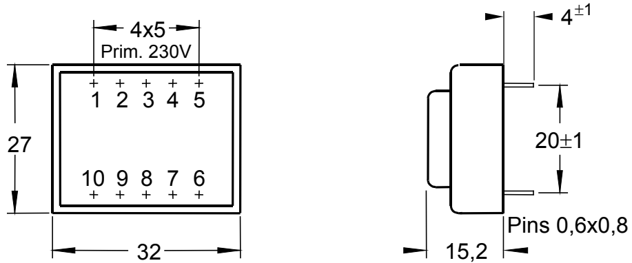
Vista lado pins / View of pins
