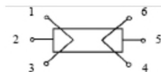
Fig8. Lead sketch
