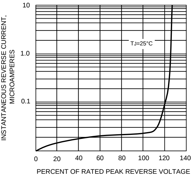
FIG.2-TYPICAL REVERSE CHARACTERISTICS
