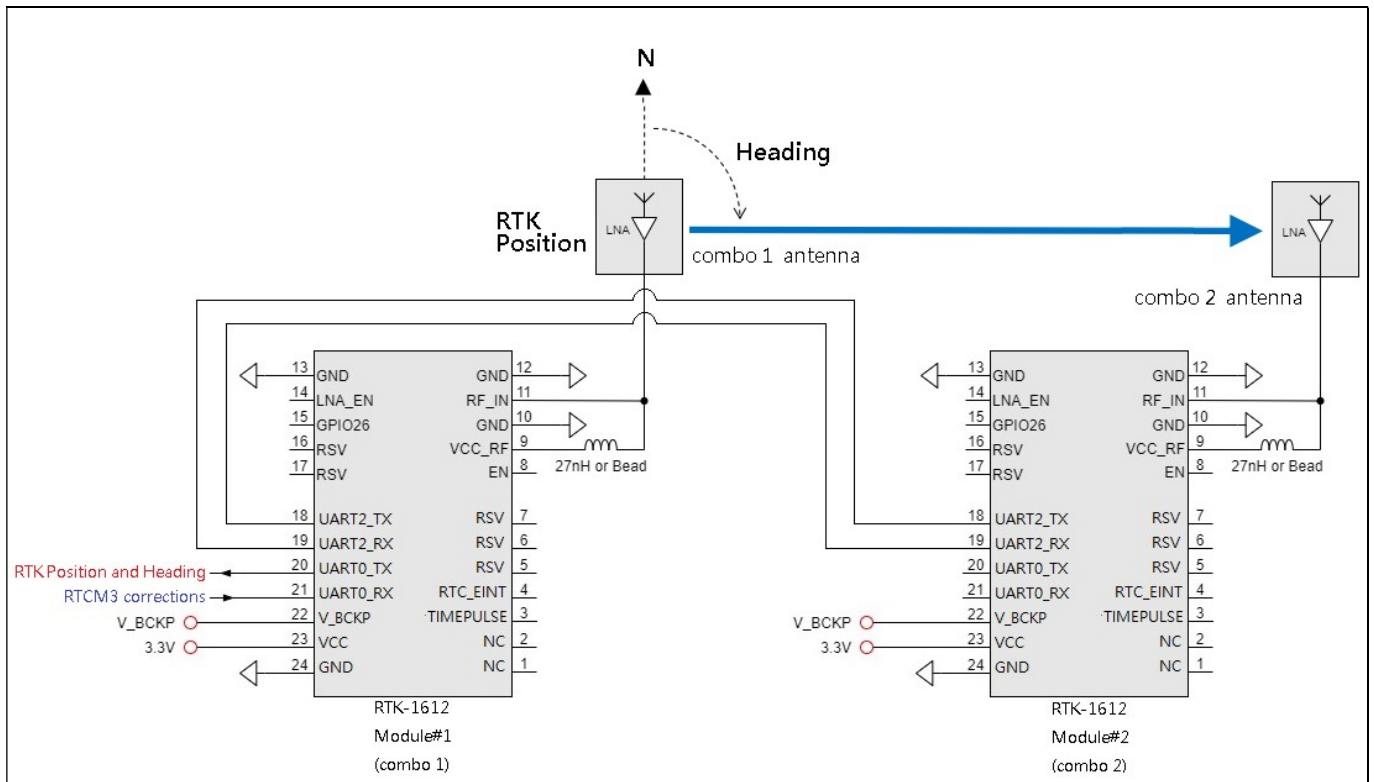
Fig 3-3 RTK-1612 (Position & Orientation) Reference Circuit
