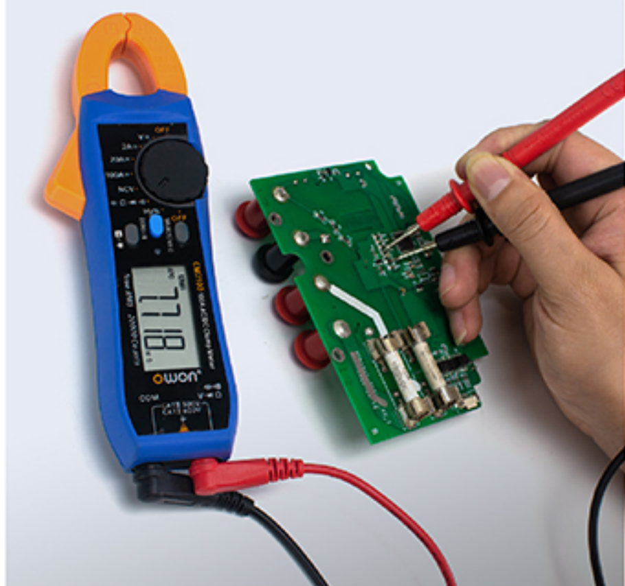
Circuit board resistance measurement
