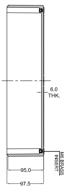
SECTION C-C
