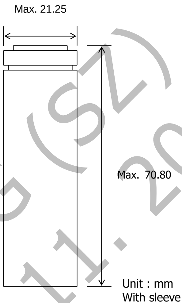
Fig. 1 Outline Dimensions of INR21700-50E
