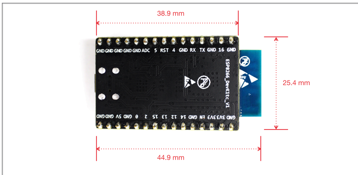
Figure 4-1. Board Dimensions
