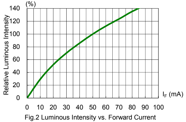
Fig.2 Luminous Intensity vs. Forward Current
