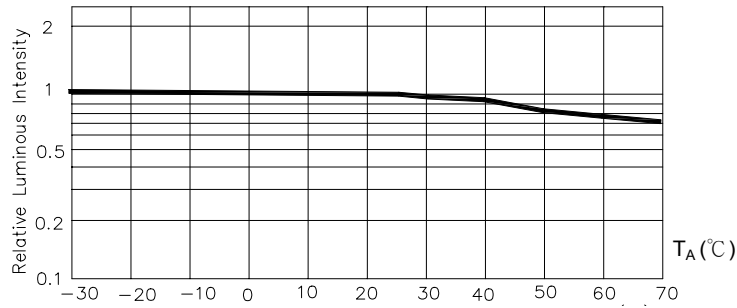
Fig.5 Luminous Intensity at I_F = 50mA vs. Ambient Temperature
