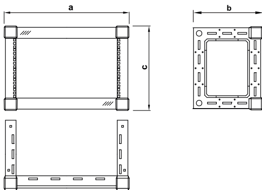
EASYRACK FRAME
