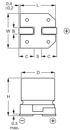
Fig.2 Dimensional outline.
