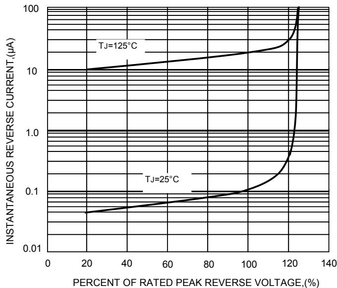
FIG.5-TYPICAL REVERSE CHARACTERISTICS
